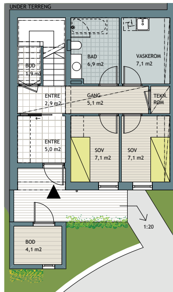
PLAN 1
