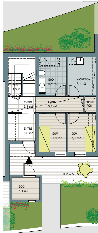
PLAN 1
